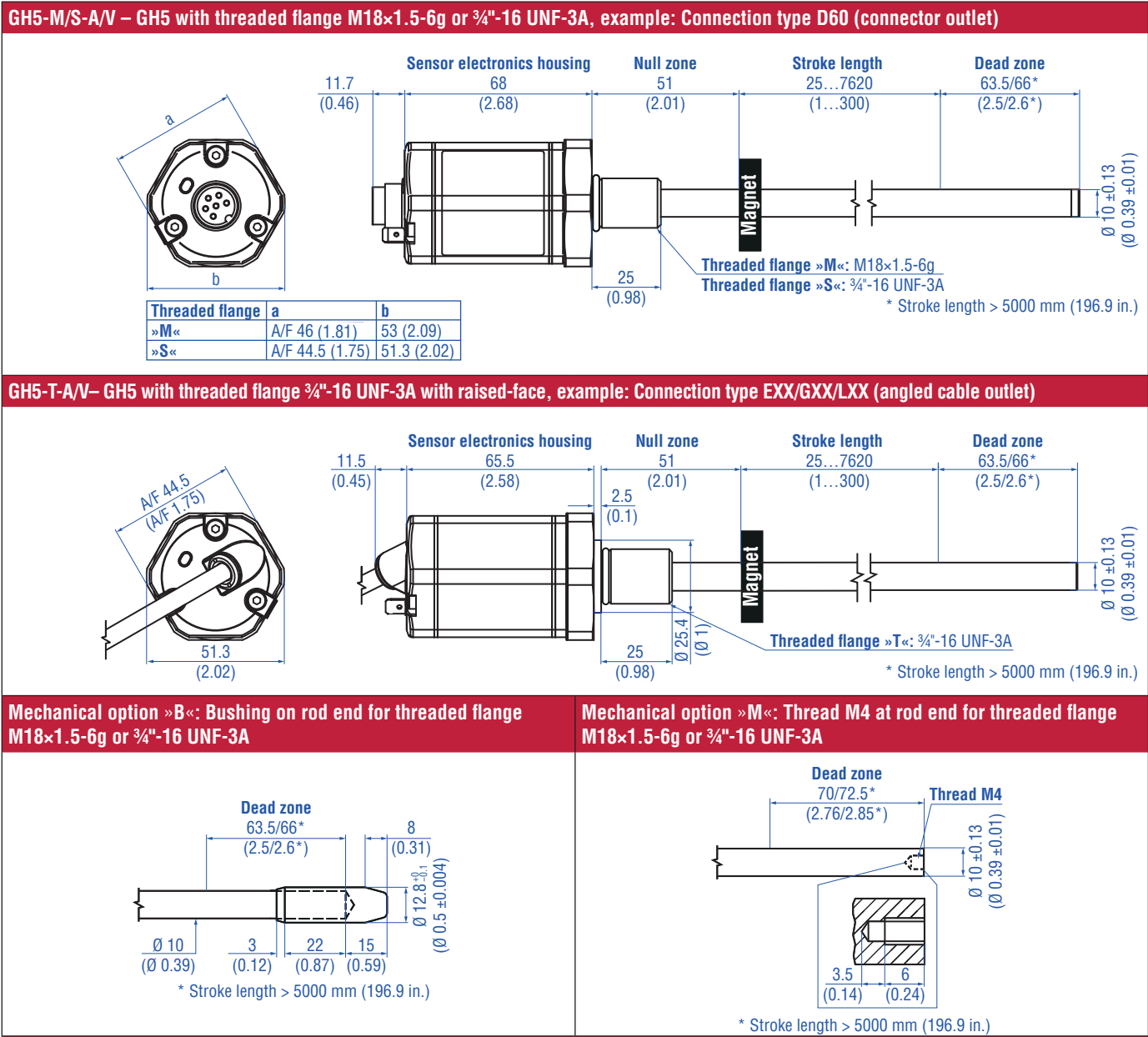
Fig. 2: Temposonics® GH5 with ring magnet
