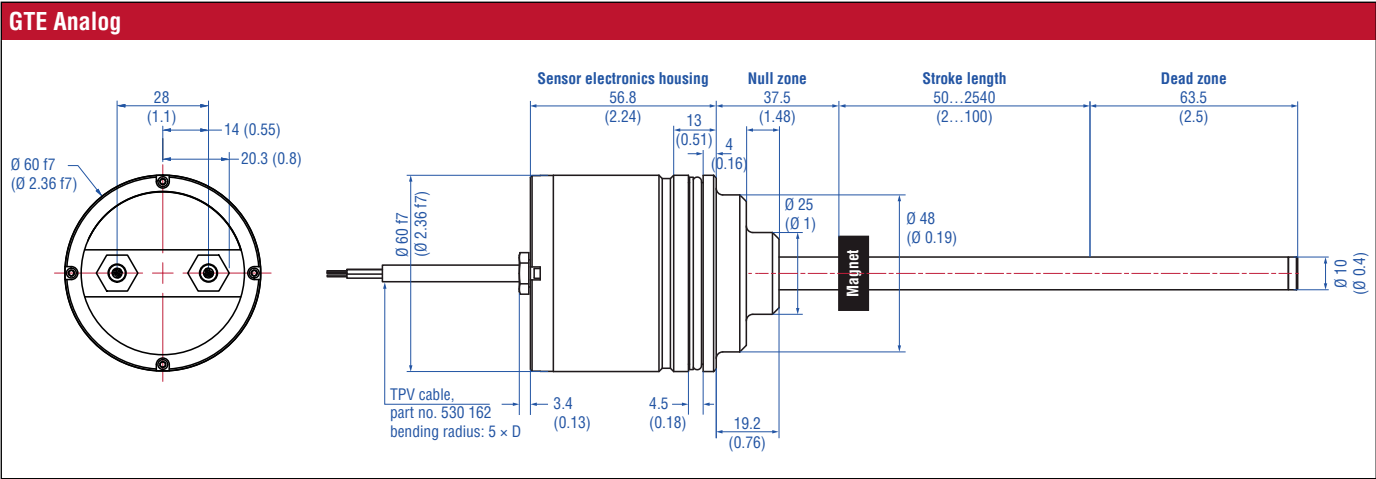
Fig. 4: Temposonics® GTE with ring magnet
