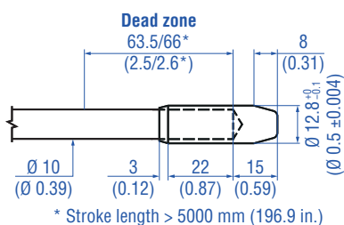
Fig. 2: Temposonics® RH5 with ring magnet, part 1
