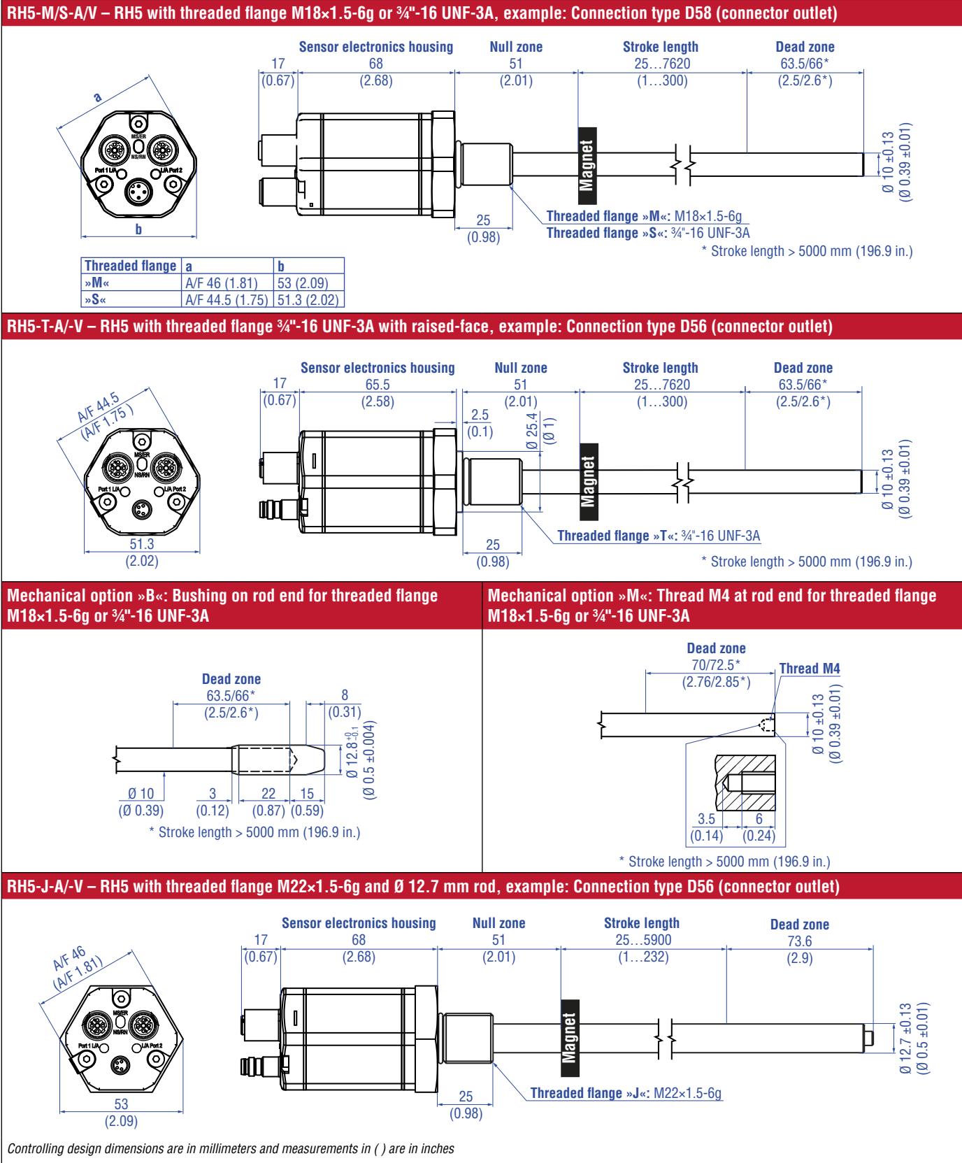
Fig. 2: Temposonics® RH5 with ring magnet
